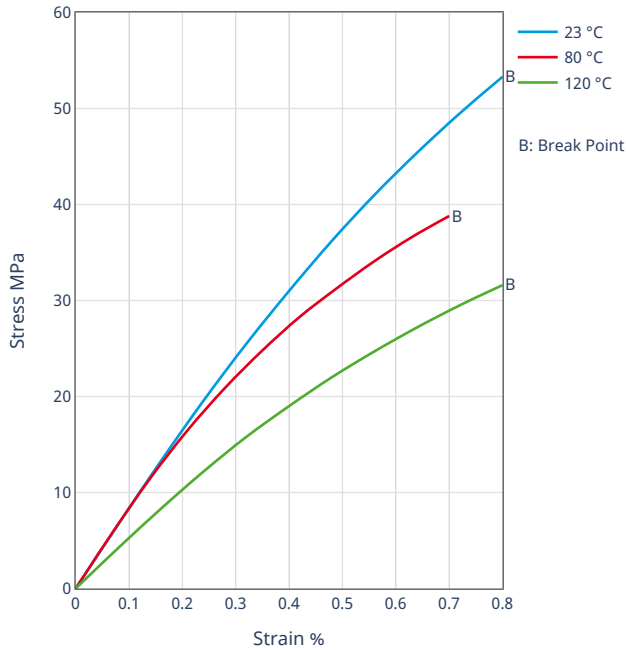
Stress-strain
